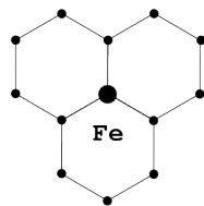
substitutional
