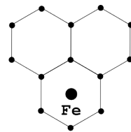
interstitial
